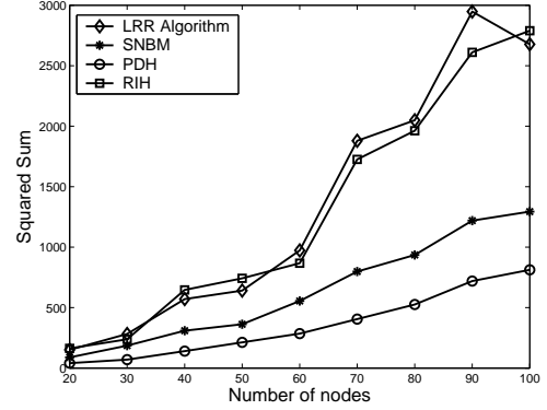
Fig. 11. SS for shortest path routing.
