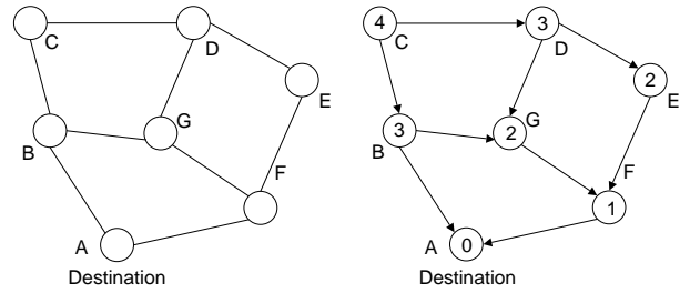
(a) Connected network graph.
