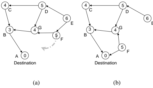
Fig. 3. An example of unequal load distribution in LRR algorithm.
