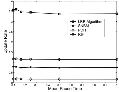
Fig. 14. Comparison of number of updates for various versions of link reversal algorithm.
