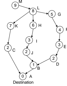
Fig. 6. A load unbalance may not always be due to selfish nodes.
