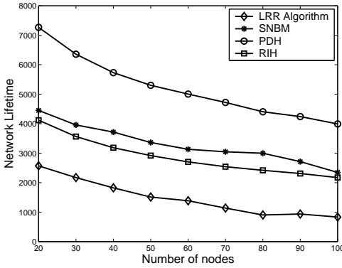
Fig. 13. Network lifetime for multipath routing.
