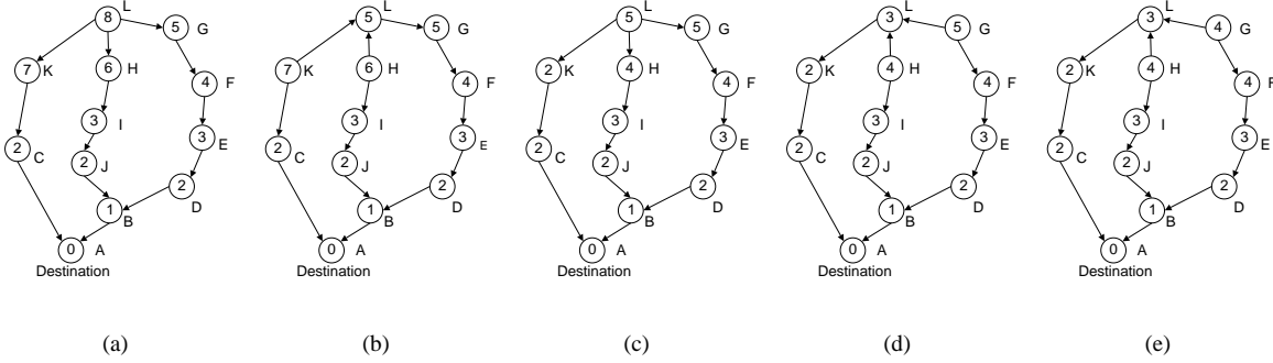
Fig. 5. An example showing how the selfish node based mechanism works.
