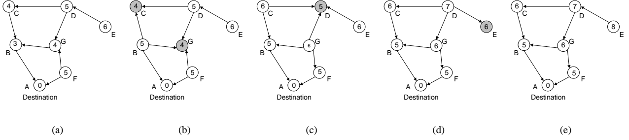
Fig. 8. An example showing how reactive increase in heights leads to load balancing.
