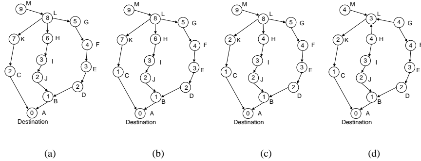
Fig. 7. An example showing how proactive decrease in height leads to load balancing.
