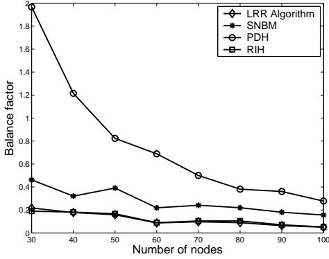
Fig. 12. BF for shortest path routing.
