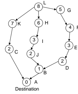
Fig. 4. A selfish node may lead to load unbalance.
