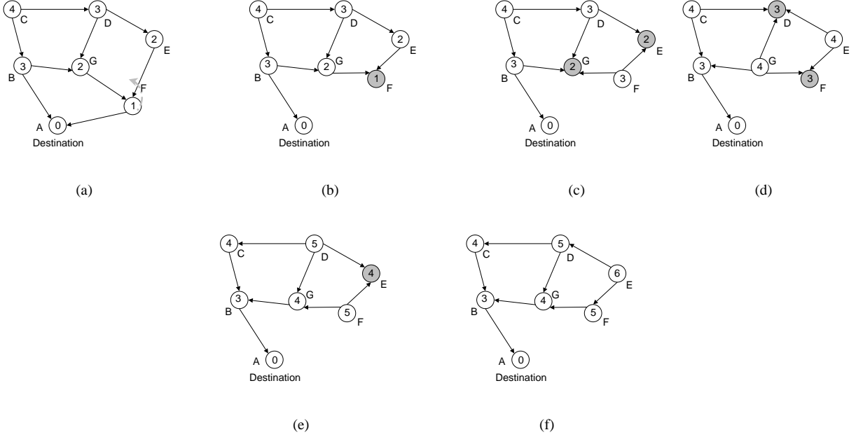
Fig. 2. Execution of full reversal algorithm. The nodes shaded gray are sinks.
