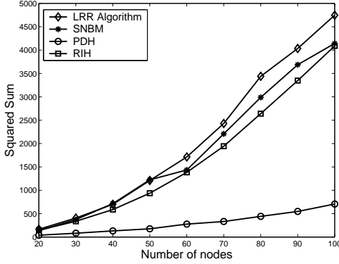
Fig. 9. SS for multi-path routing.
