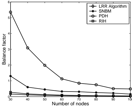
Fig. 10. BF for multi-path routing.
