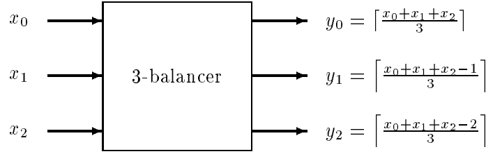
Figure 2: A 3-balancer
